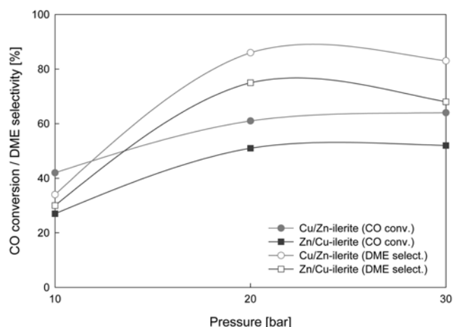
Fig. 6. Effect of pressure on CO conversion and DME selectivity for direct DME synthesis from syngas over M/M-ilerite (M: Cu, Zn) catalysts at 250^\circ\text{C} , \text{H}_2/\text{CO}=2 .
