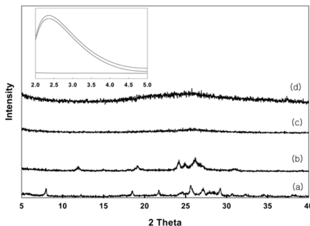
Fig. 1. XRD patterns of prepared ilerite catalysts: (a) Na-ilerite, (b) H-ilerite, (c) Cu-ilerite, (d) Cu/Zn-ilerite.
