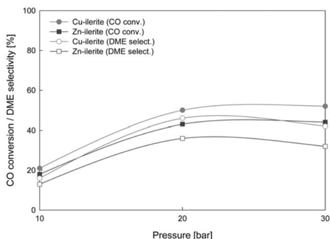
Fig. 5. Effect of pressure on CO conversion and DME selectivity for direct DME synthesis from syngas over M-ilerite (M: Cu, Zn) catalysts at 250^\circ\text{C} , \text{H}_2/\text{CO}=2 .
